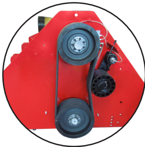
Tendicinghia automatico Automatic belt tightener
